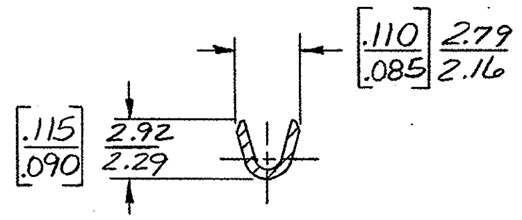
SECT. B-B
